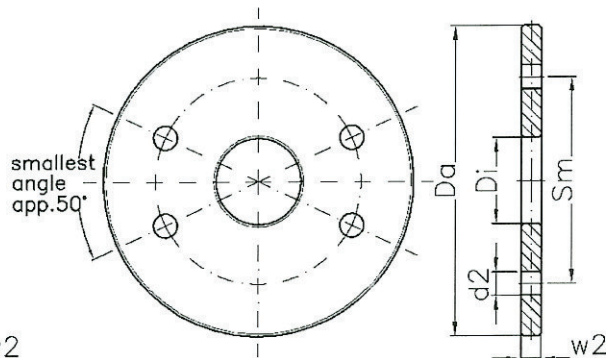
anchor disc made of steel
