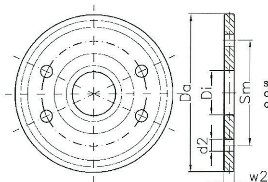
anchor disc made of cast iron
