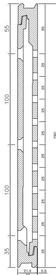
COUPLED CONNECTORS
