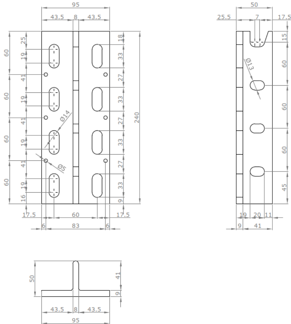
Drawing: ALUMEGA 240 HV
