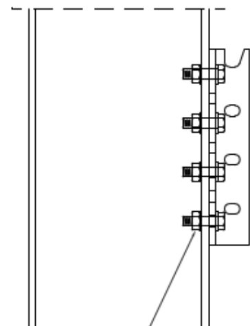
M12 steel bolt
