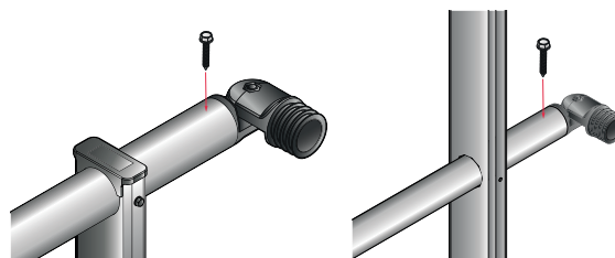
14 - Fasten the angle brackets with 4,8 x 25 self-drilling screws.
