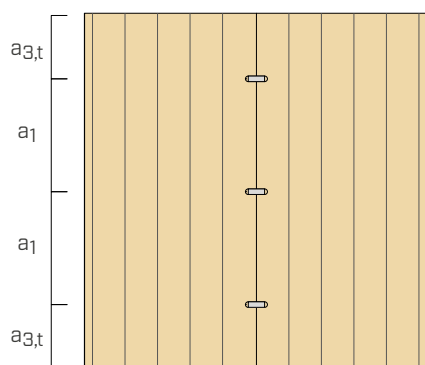
SHEAR WALL
