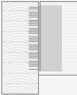
Main-secondary joint with AluMIDI bracket.
