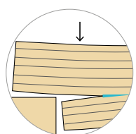
NOTCH tension reinforcement perpendicular to grain
