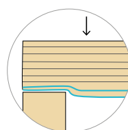
SUPPORT compression reinforcement perpendicular to grain
