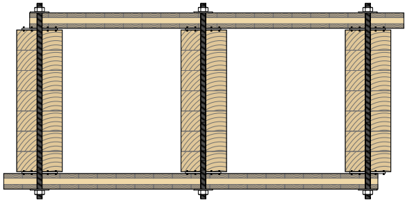
fastening with threaded rods or bolts
