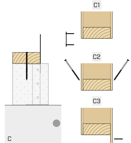
C TC FUSION WITH BASE PLATE
