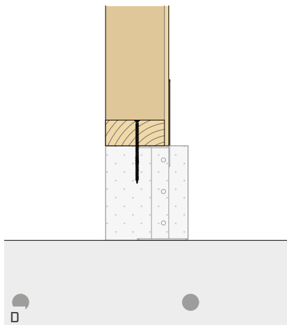
D TC FUSION WITH TOP INSERTION
