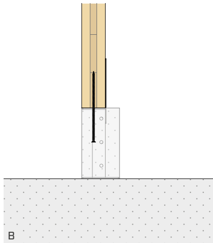
B TC FUSION WITH BOTTOM INSERTION
