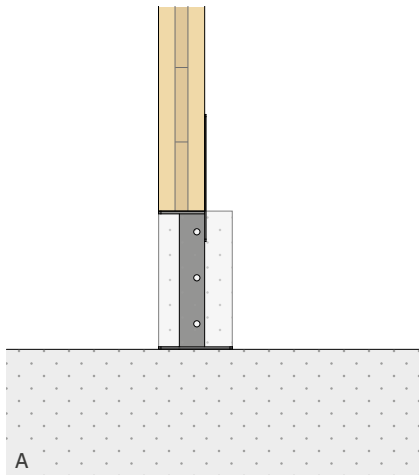
A UP LIFT
