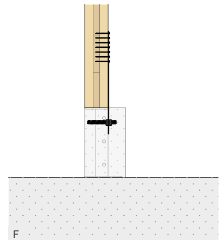
F WHT PLATE C
