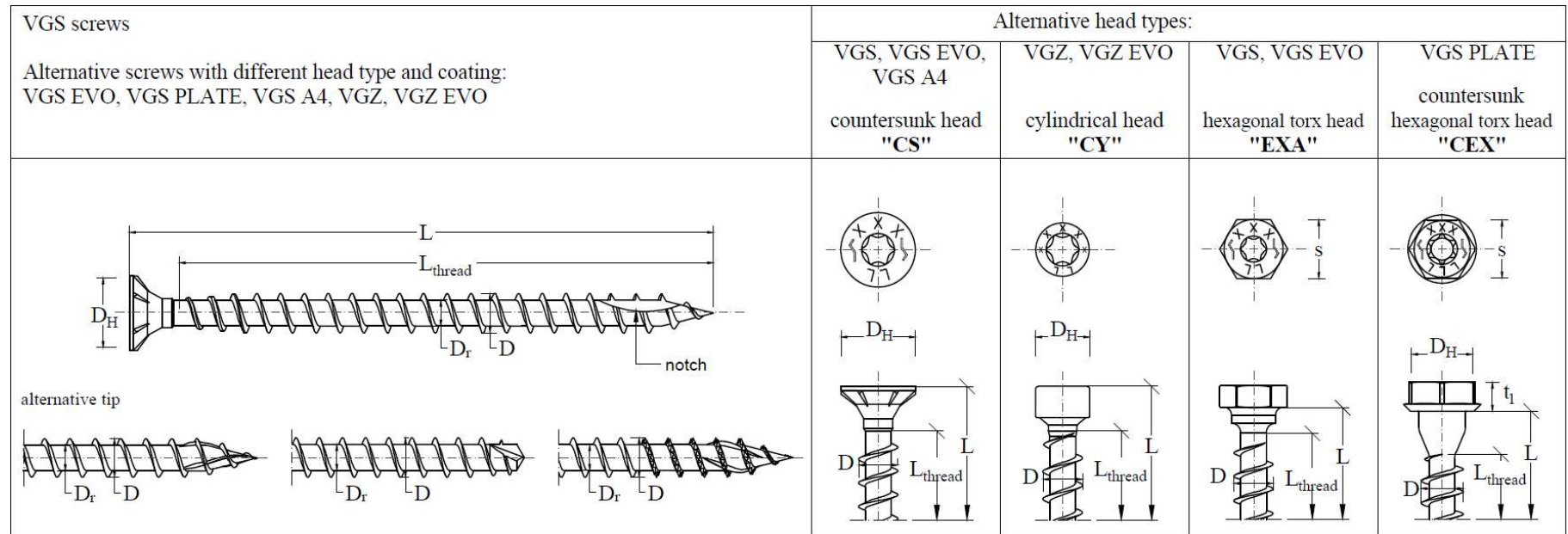
FIGURE 3—TYPICAL VGS, VGS EVO, VGS PLATE, VGS A4, VGZ AND VGZ EVO FULLY THREADED SCREWS
