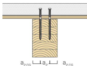
30°/45° parallelle
