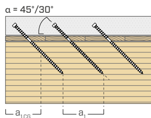
30°/45° parallelle
