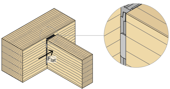
LOCK STOP
