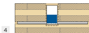
4 During the storage or transport of elements, MANTIS can remain protected in the hole
