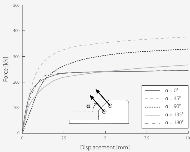
Force-displacement diagram
