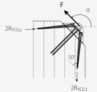
Configuration for \alpha = 135^\circ - 315^\circ
