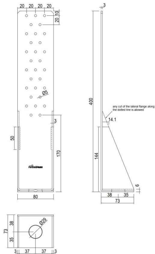
Figure B.3 Dimensions of Rotho Blaas WHT30 hold down.
