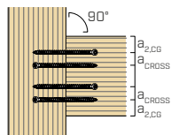
plan - 2 OR MORE PAIRS
