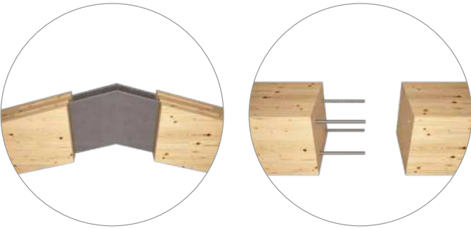
1. MOMENT CONTINUITY JOINT
