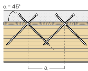
45° crossed
