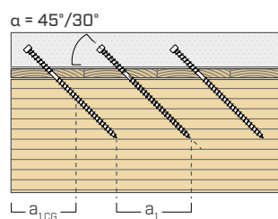
parallel at 30°/45°
