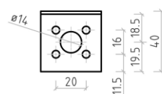
Figure B. 4 Dimensions of type WZU 3002
