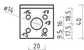
Figure B. 3 Dimensions of type WZU 2004
