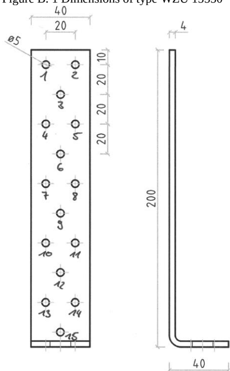
Figure B. 1 Dimensions of type WZU 15550
