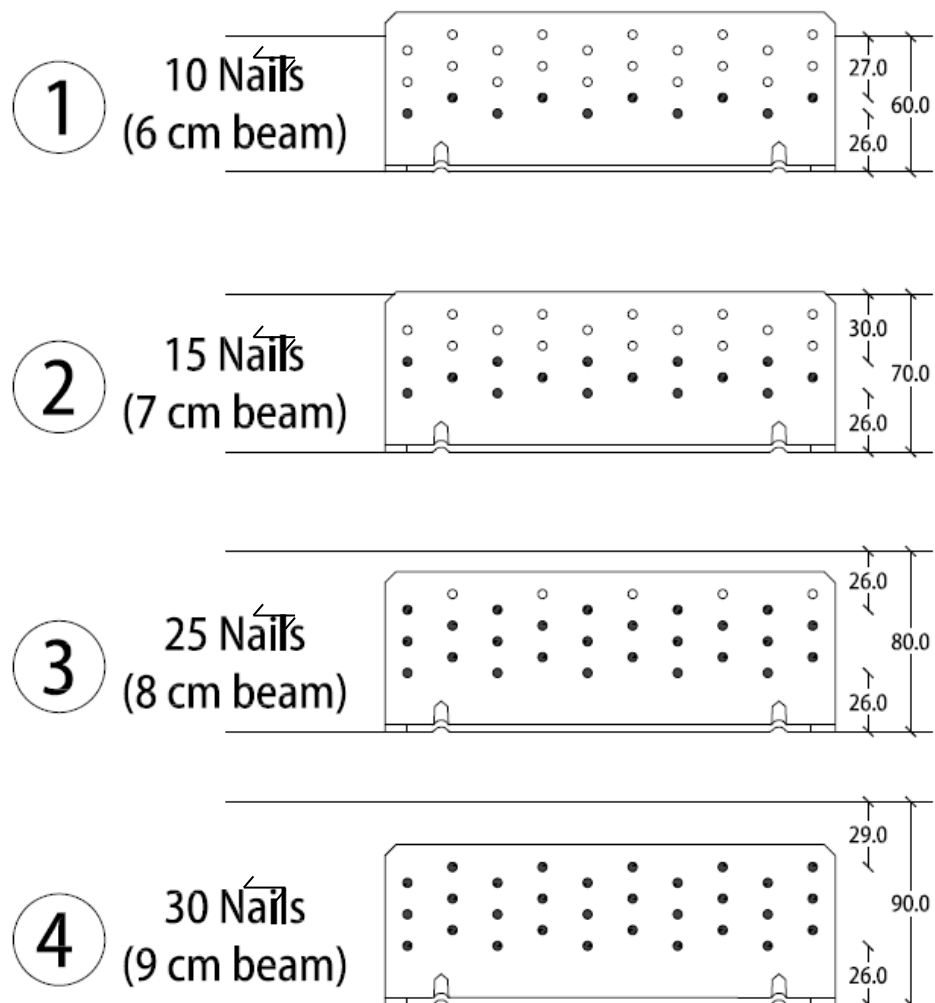
Figure B. 18 Typical installation for Angle Bracket TITAN TTF200 and TCF200 (for TTF200: symmetrical hole-pattern for horizontal and vertical flange)
