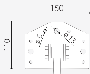
ANCHOR PLATE
