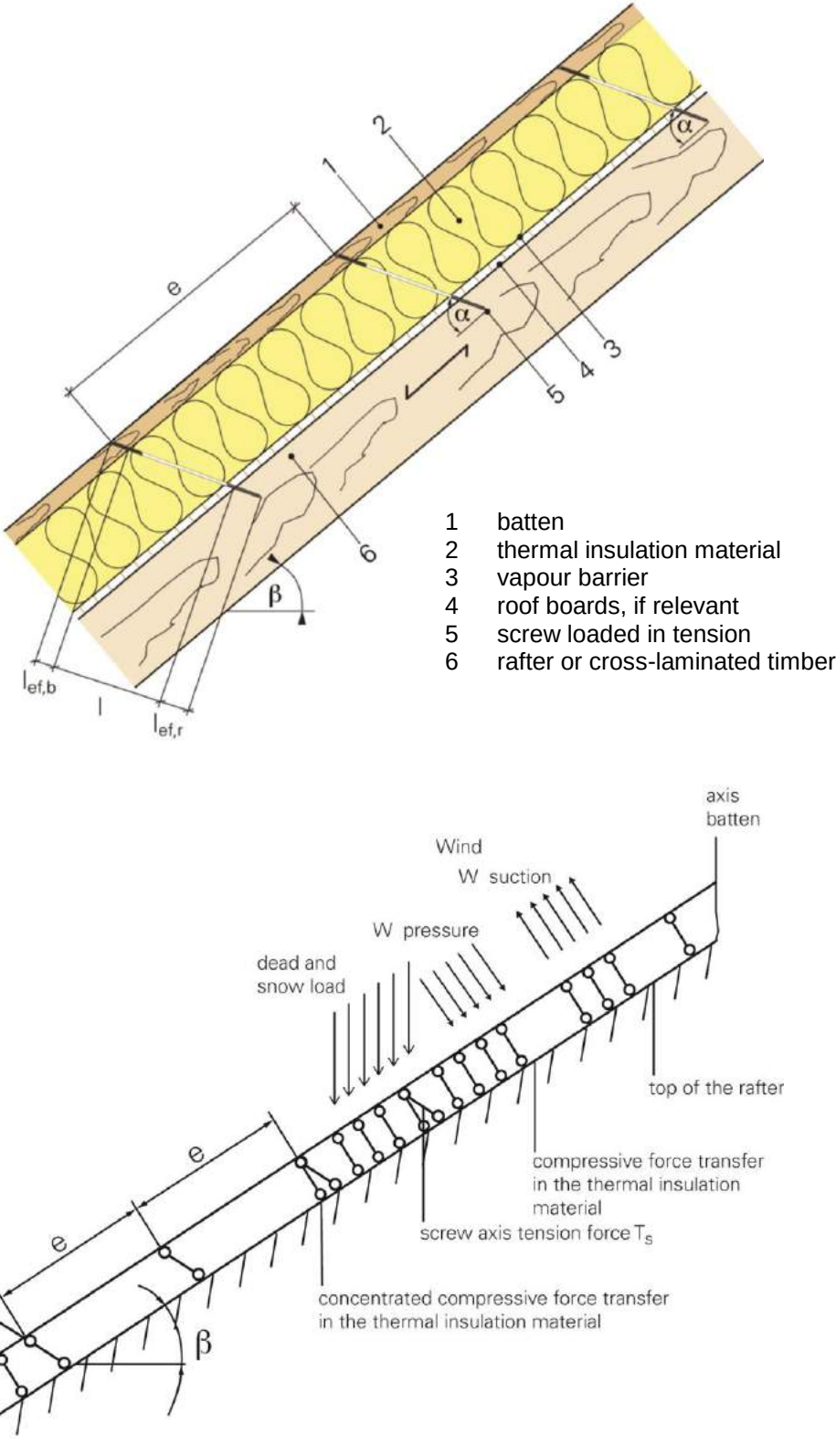
Figure A.3.1 Fastening of the thermal insulation material on top of rafters - structural system
