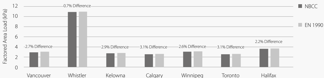
Figure A.2: Comparison of NBCC & EN Factored Loads - Sloped Roof
