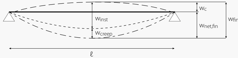
Figure 4: Vertical deflections
