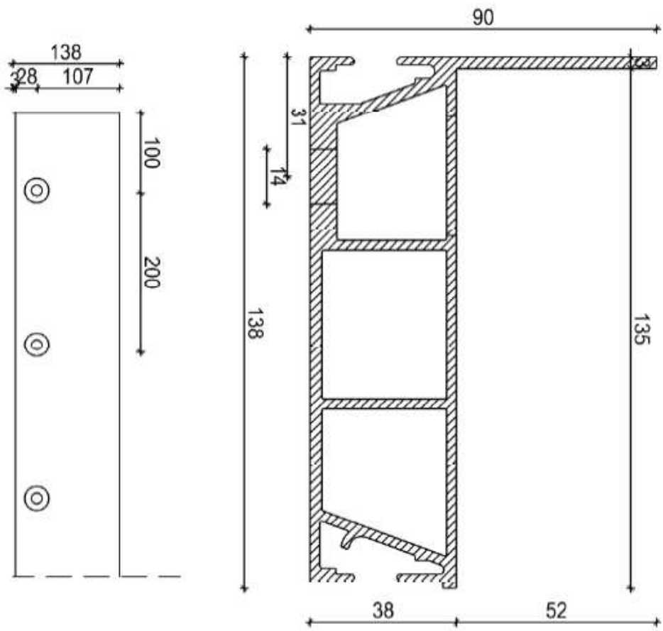
Figure C.7: ALU START 135 – Longitudinal section and top view
